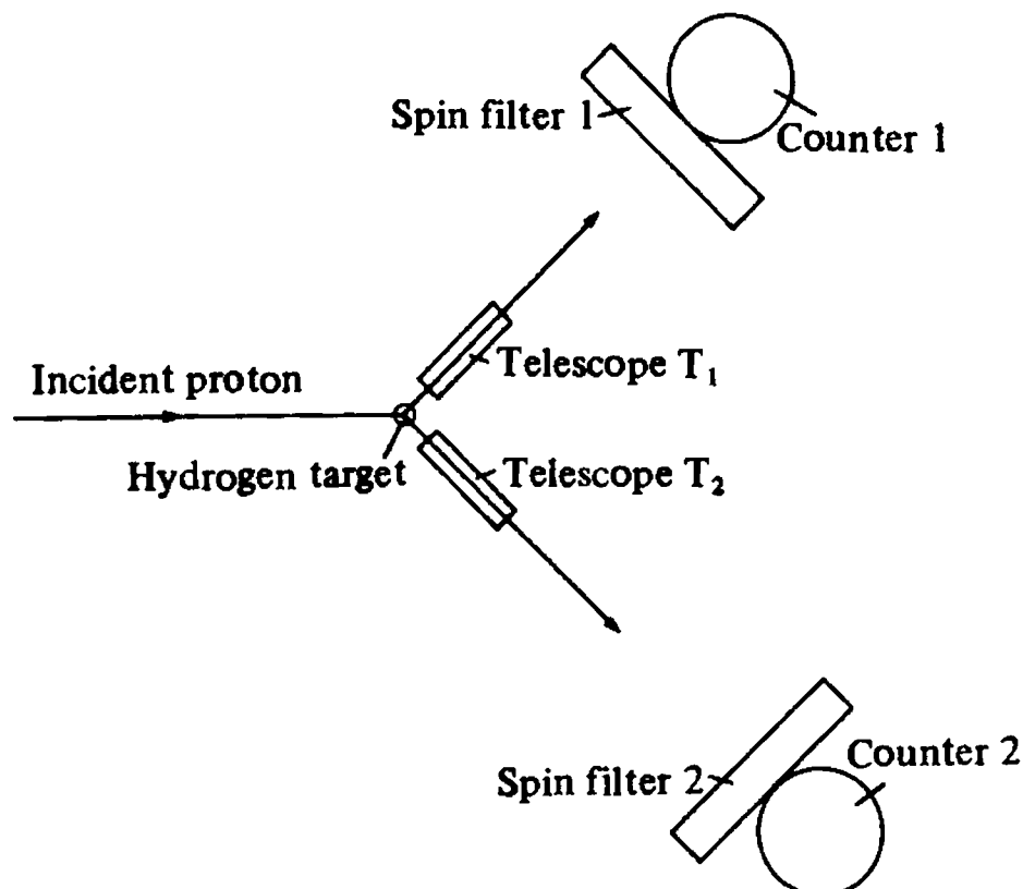
Fig. 1. Proton–proton scattering gedanken experiment.
